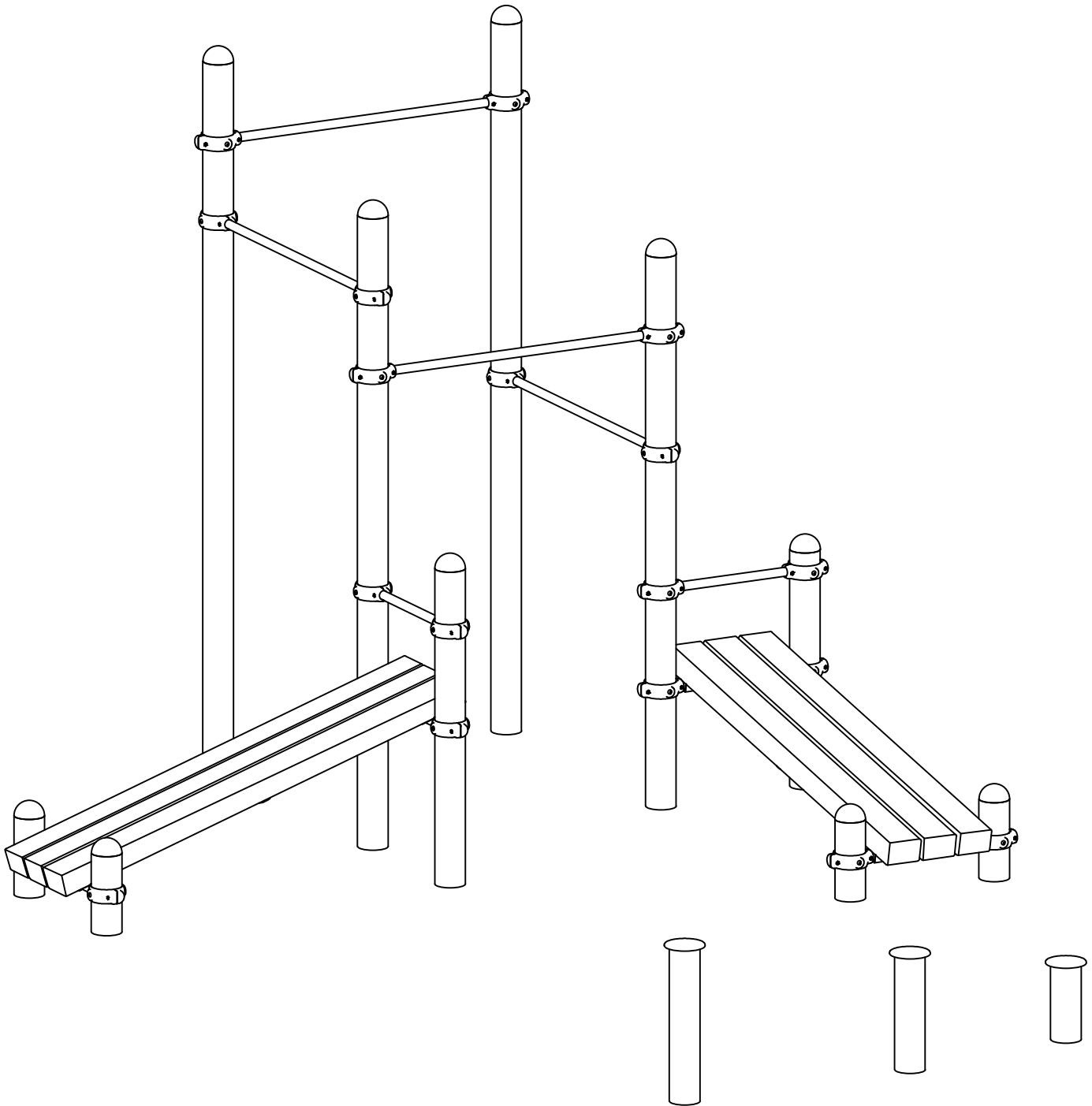
ISOMETRIC VIEW
