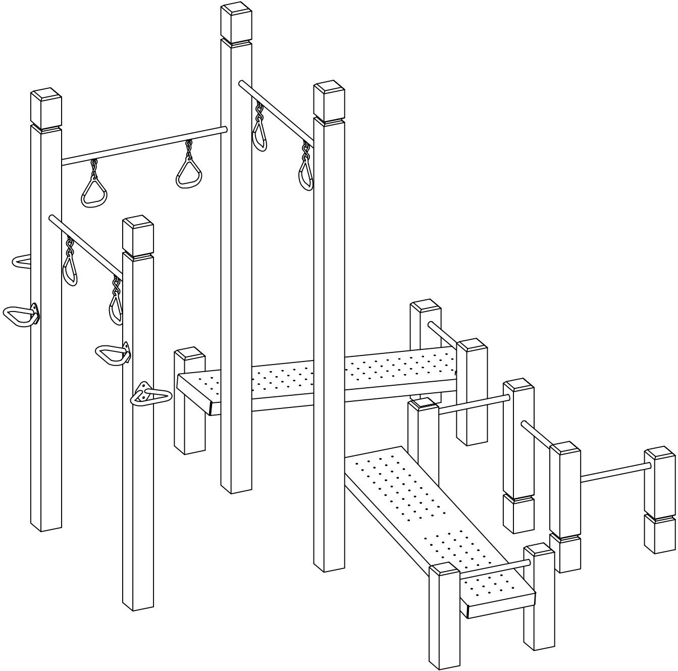
ISOMETRIC VIEW
