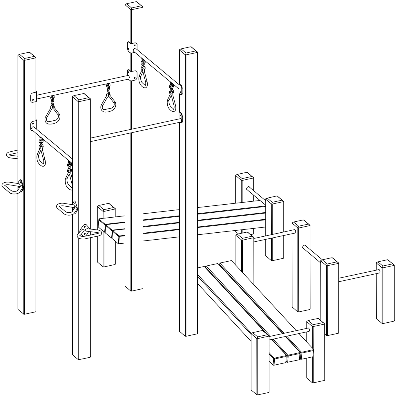
ISOMETRIC VIEW
