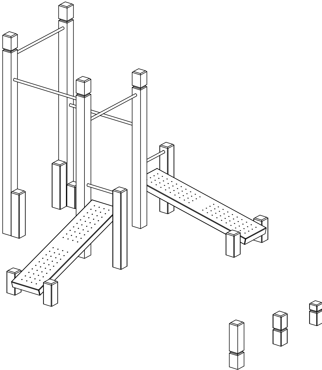
ISOMETRIC VIEW
